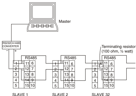
CONNECTION DIAGRAM
