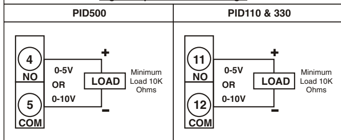
Fig5. Output 1 - Linear voltage.
